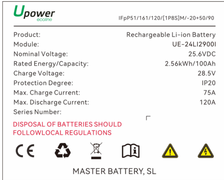
Figure 1-1 Battery Energy Storage System nameplate
